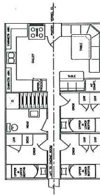
LOWER DECK
